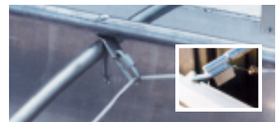
Top: Bows swing back and up; bow in angled bracket; and center pivoting ridge pole with locking system [inset].
